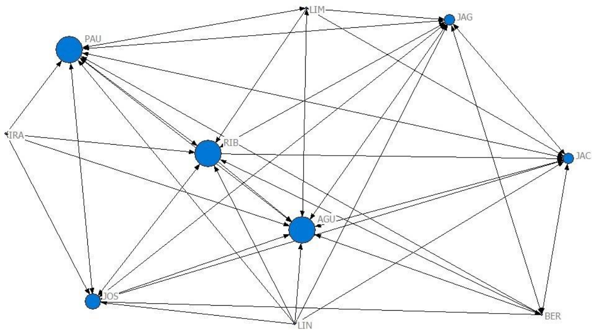
Figure 5. Closeness centrality
