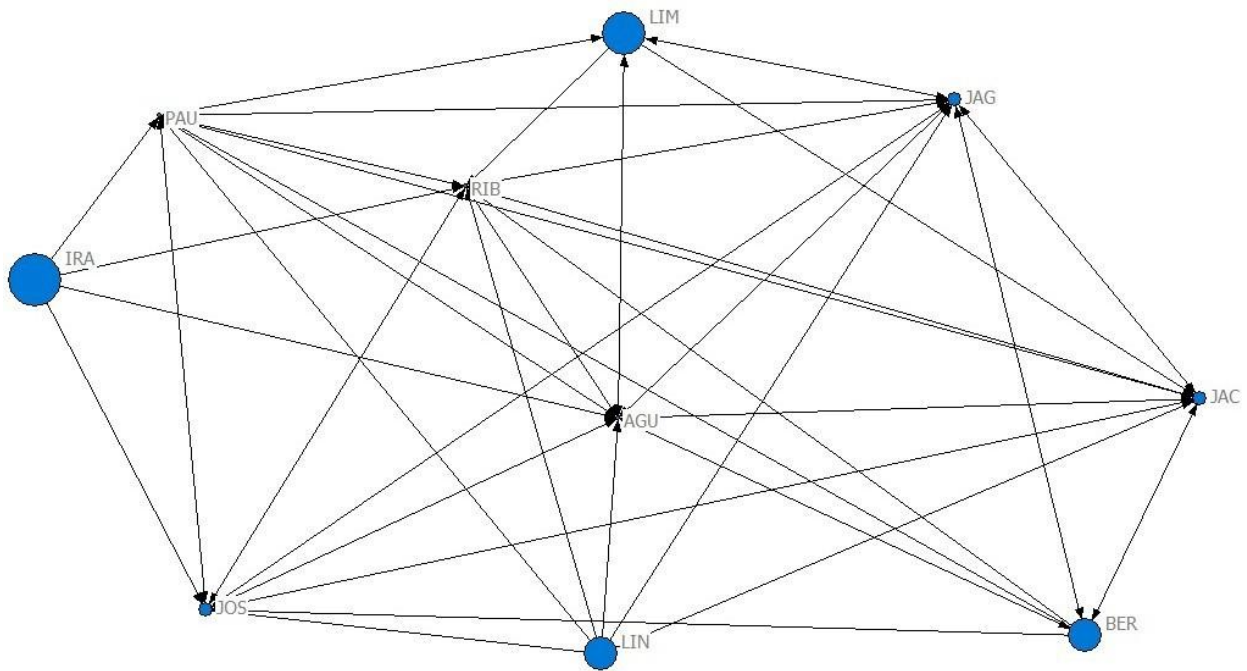
Figure 4. Betweenness centrality
