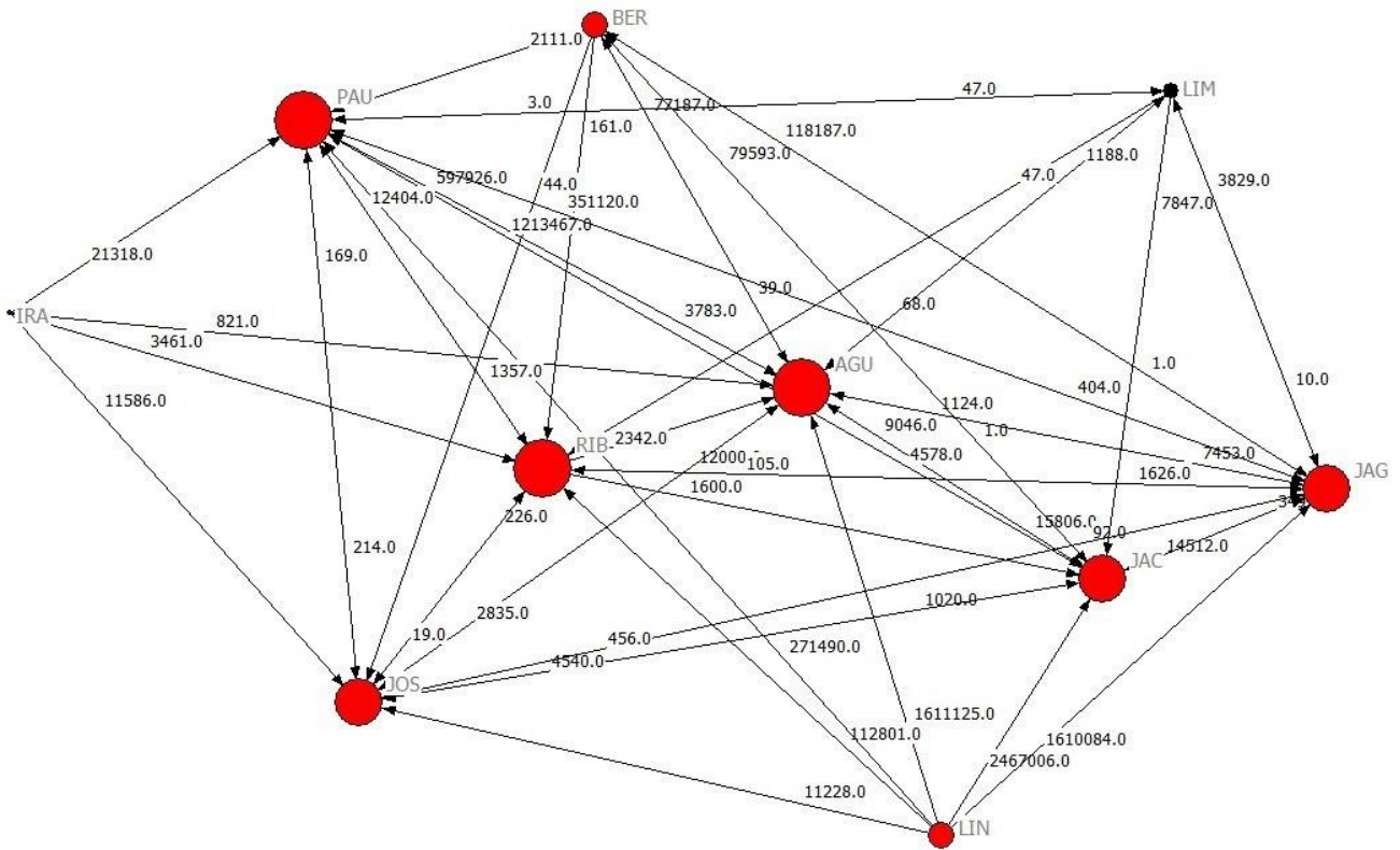
Figure 6. K-core
